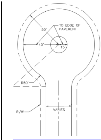
STANDARD TURNING AREA (C)
