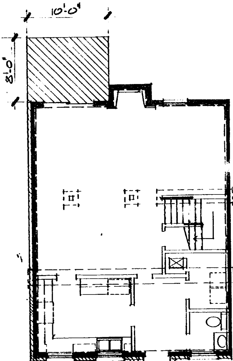
FIRST FLOOR PLAN 805# 1/8" = 1'-0"
