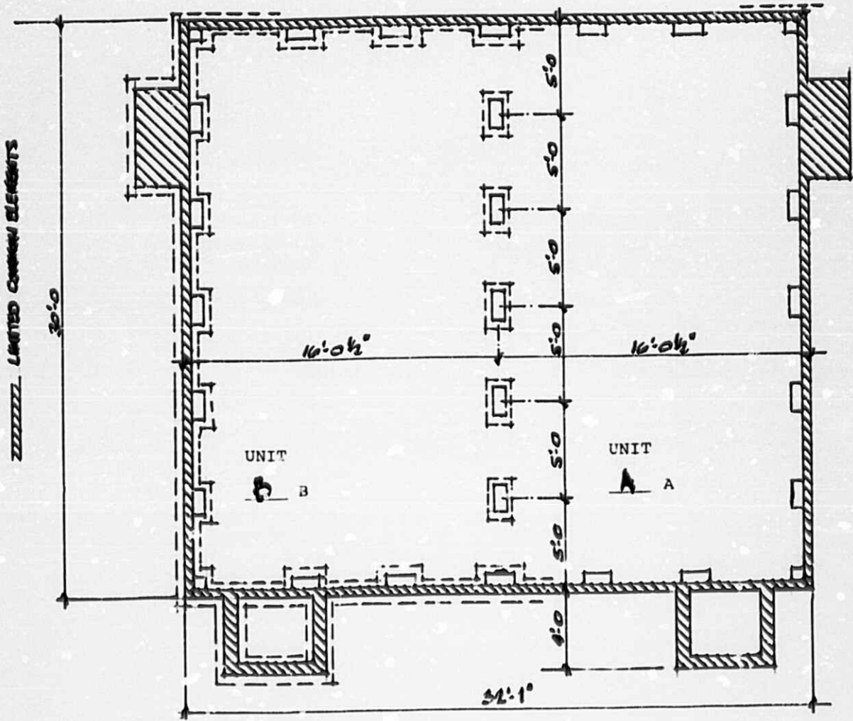
FOUNDATION PLAN
