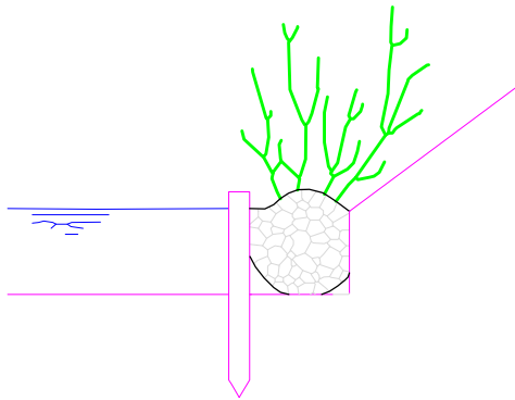
(a) FASCINE ROLL
