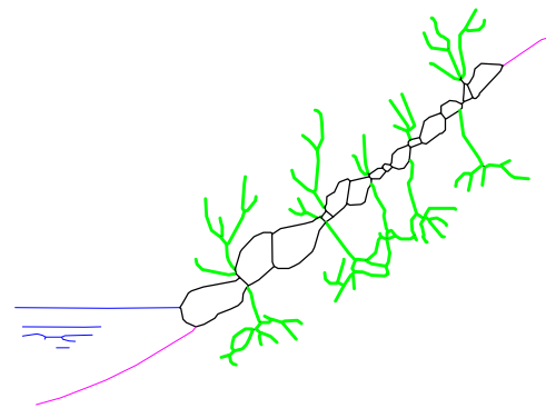
(d) CUTTINGS BETWEEN RIPRAP
