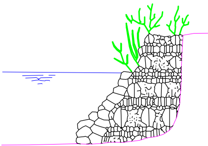
(c) PACKED FASCINE WORK
