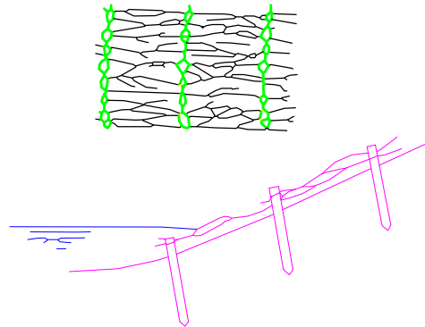
(b) WILLOW MATTRESS
