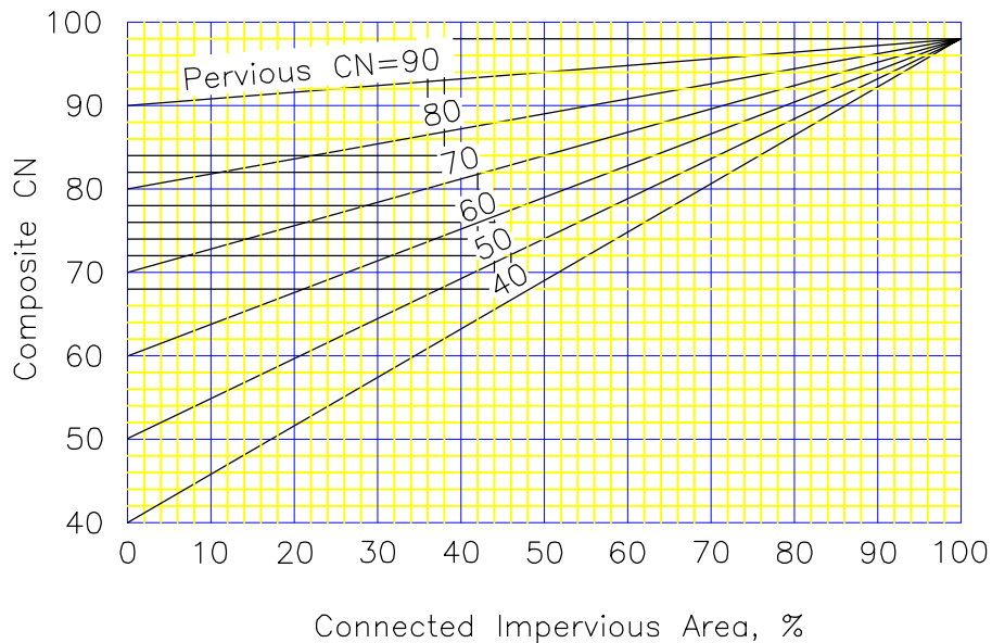
Composite CN With Connected Impervious Areas
