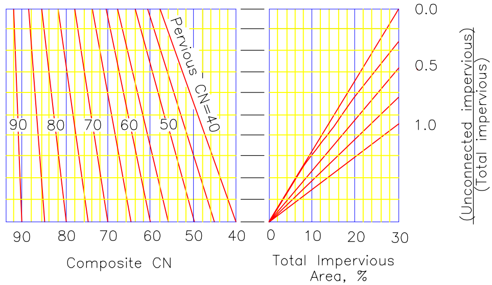
Composite CN With Unconnected Impervious Areas (Total Impervious Area Less Than 30%)
