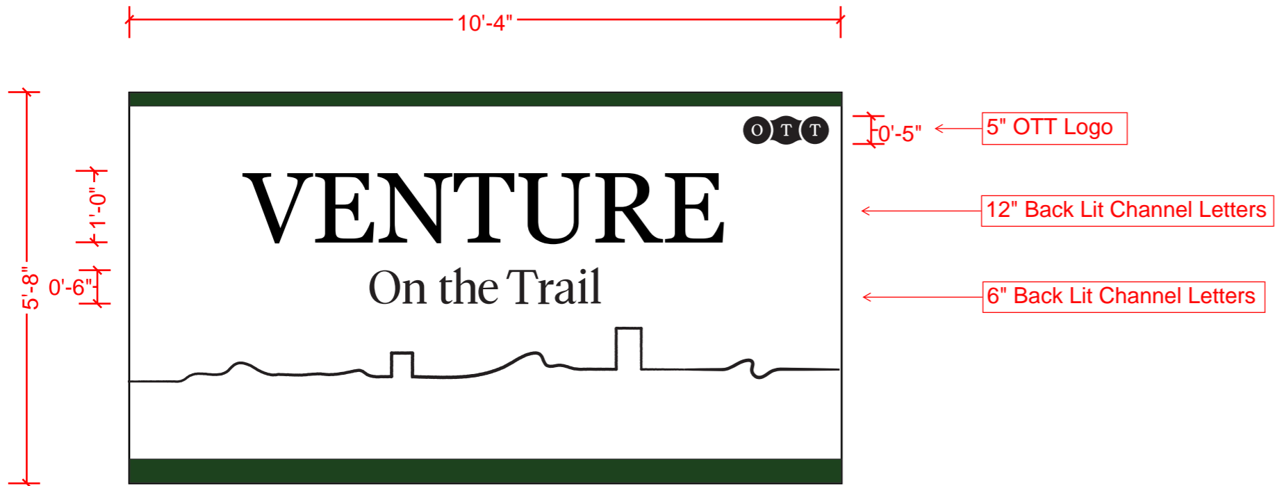
SIGNAGE 1: MAIN ENTRY MONUMENT ELEVATION NTS
